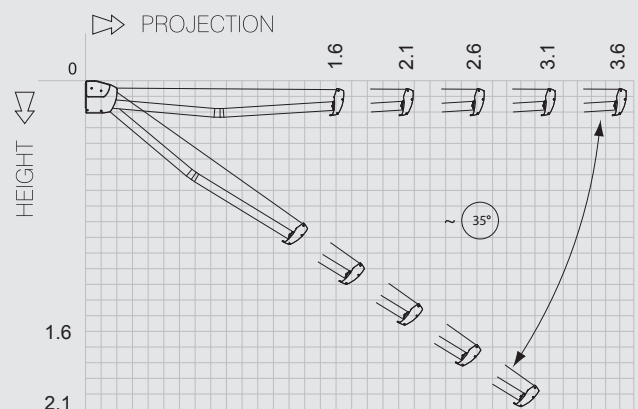
Tilt angle adjustment
